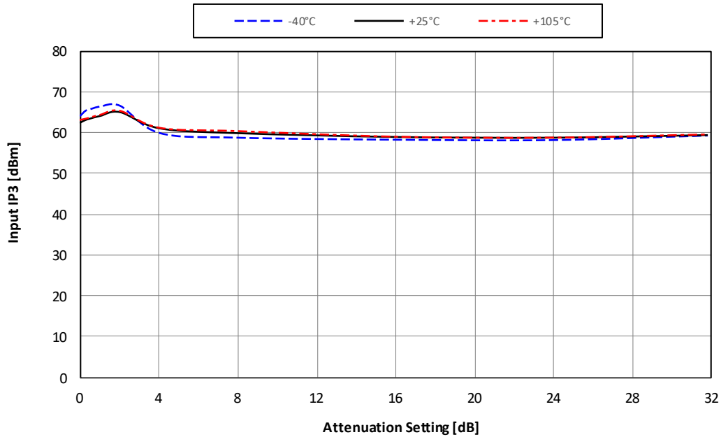
Figure 22. IIP3 @ 2500MHz vs Temperature
