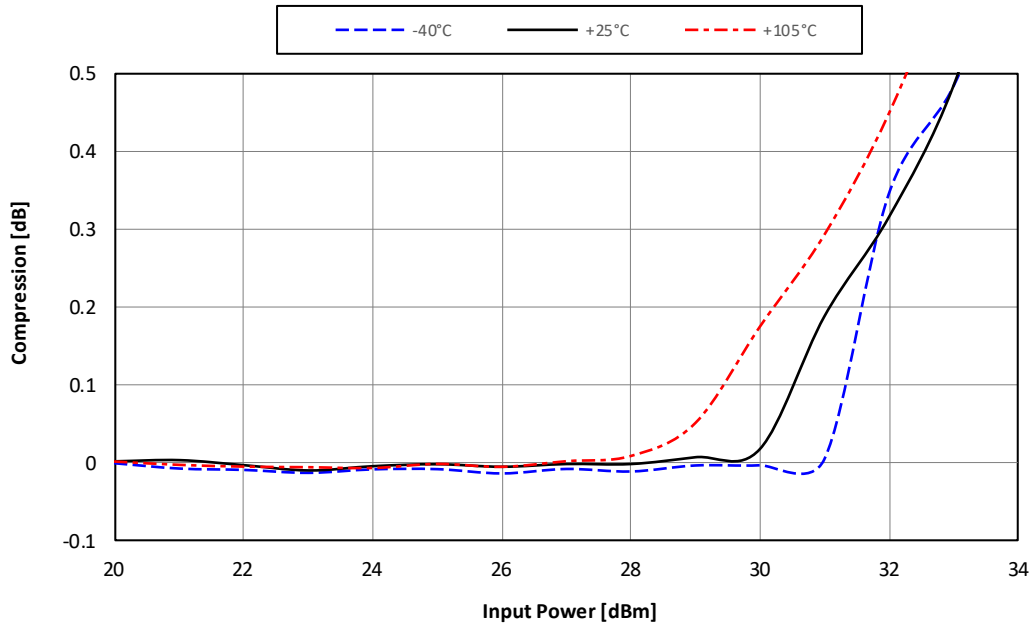
Figure 28. Input 0.1dB Compression @3500MHz vs Temperature
