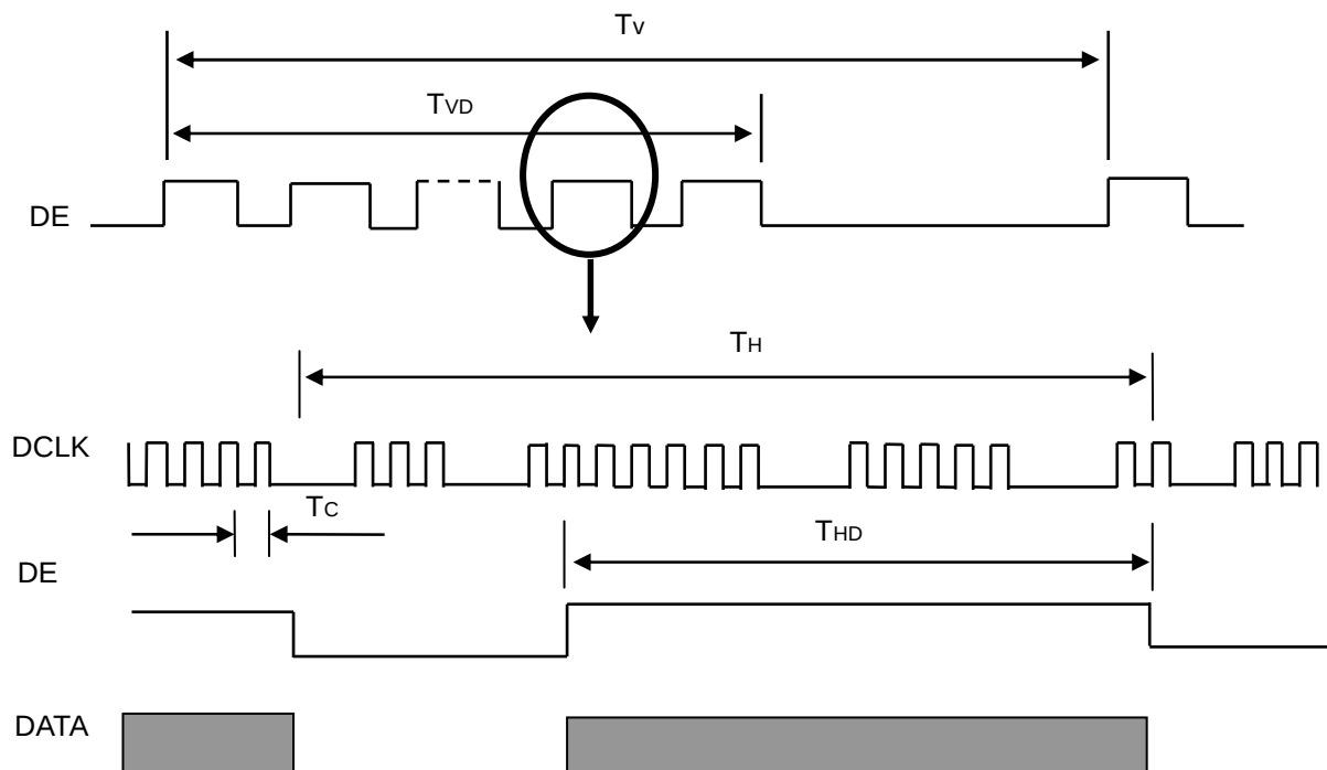
INPUT SIGNAL TIMING DIAGRAM
