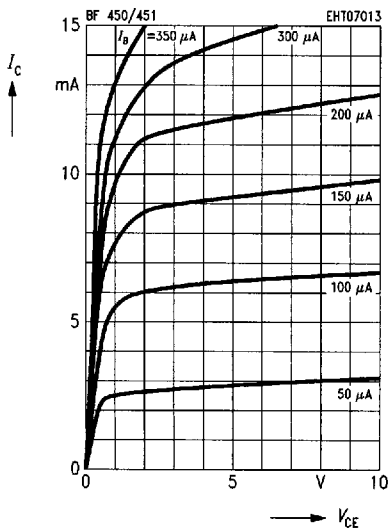
Output characteristics I_C = f(V_{\text{CE}})
