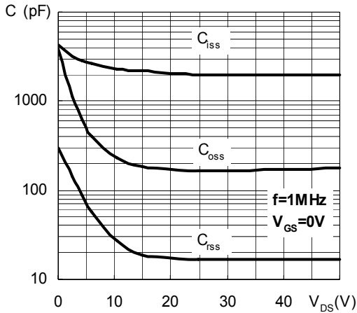
Figure 7 Capacitance
