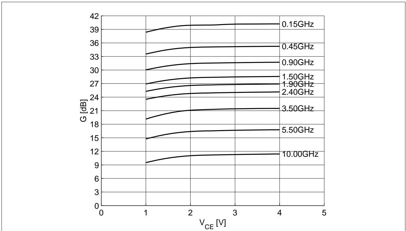
Figure 5-12 Maximum Power Gain G_{max} = f(V_{CE}) , I_C = 30 mA, f = Parameter in GHz
