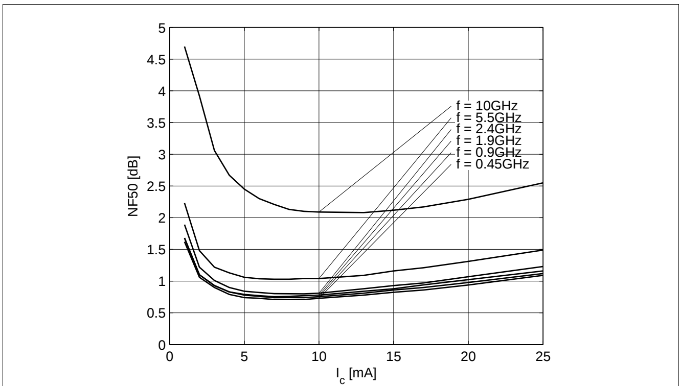
Figure 5-18 Noise Figure NF_{50} = f(I_c) , V_{CE} = 3 V, Z_S = 50 \Omega , f = Parameter in GHz
