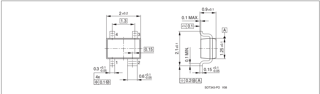
Figure 7-1 Package Outline
