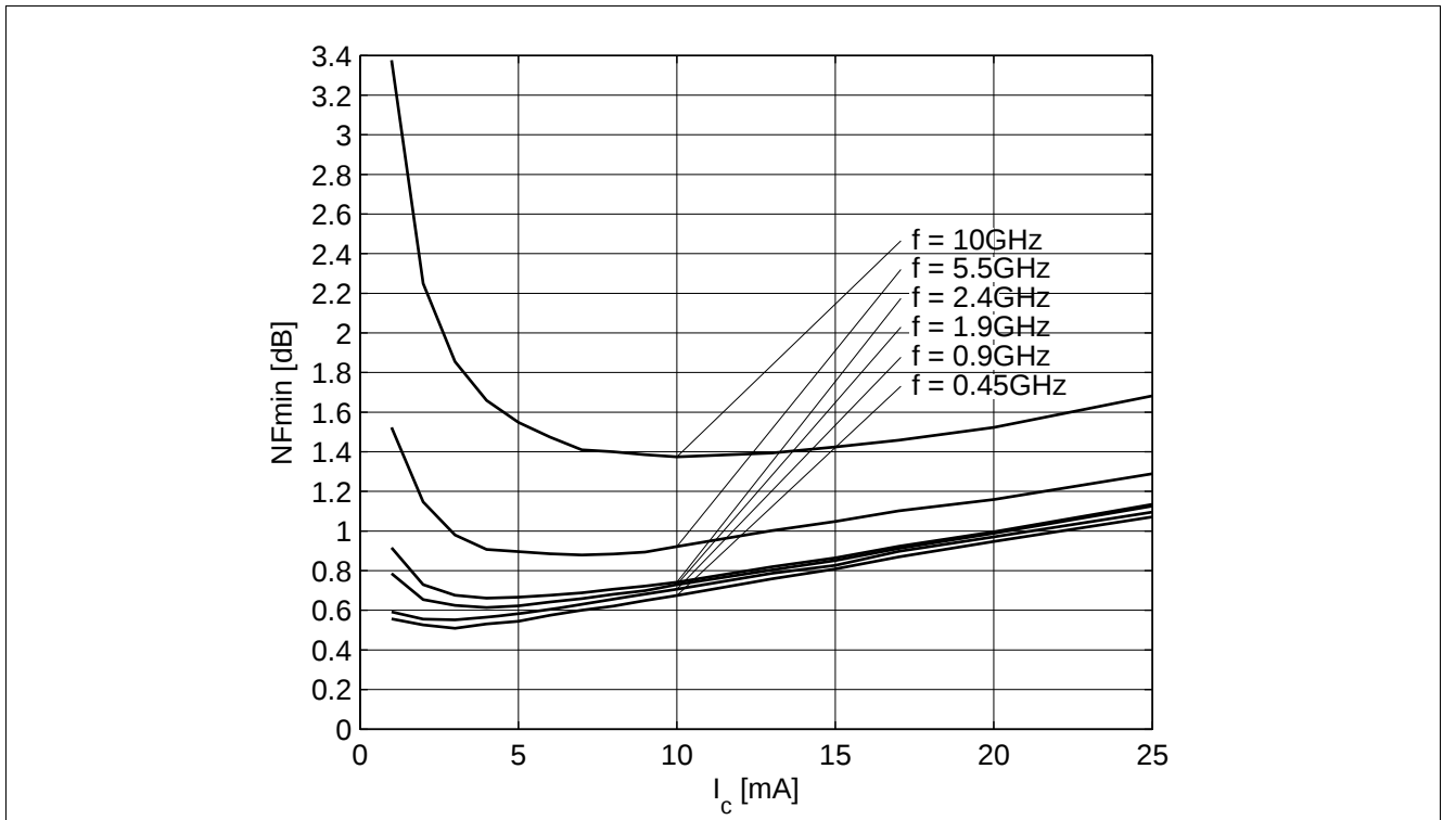
Figure 5-17 Noise Figure NF_{min} = f(I_c) , V_{CE} = 3 V, Z_S = Z_{opt} , f = Parameter in GHz
