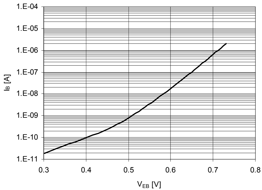
Figure 5-6 Base Current vs. Base Emitter Reverse Voltage I_B = f(V_{EB}) , V_{CE} = 2\text{ V}
