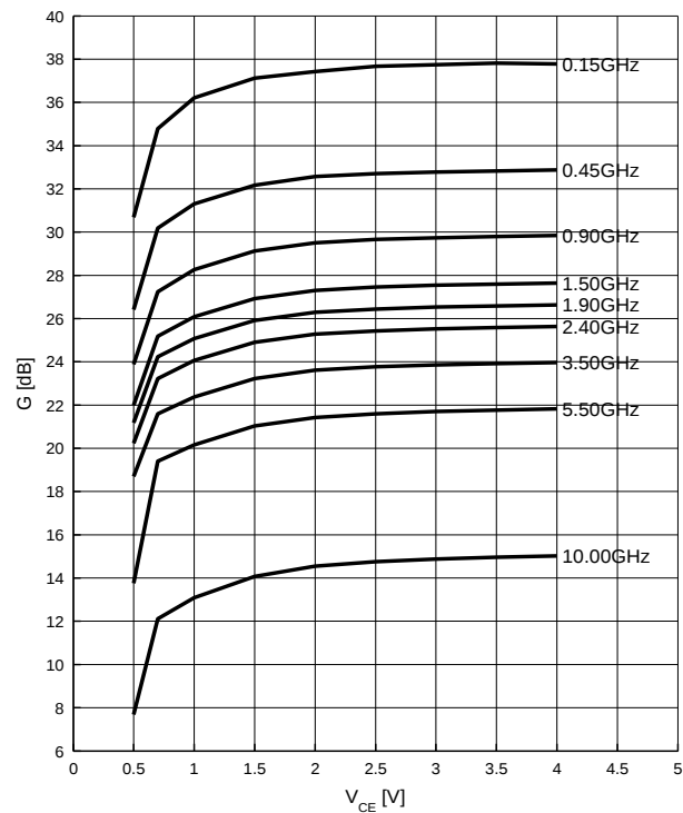
Figure 5-5 Power Gain G_{ma} , G_{ms} = f(V_{CE}) , I_C = 13\text{ mA} , f = \text{Parameter in GHz}
