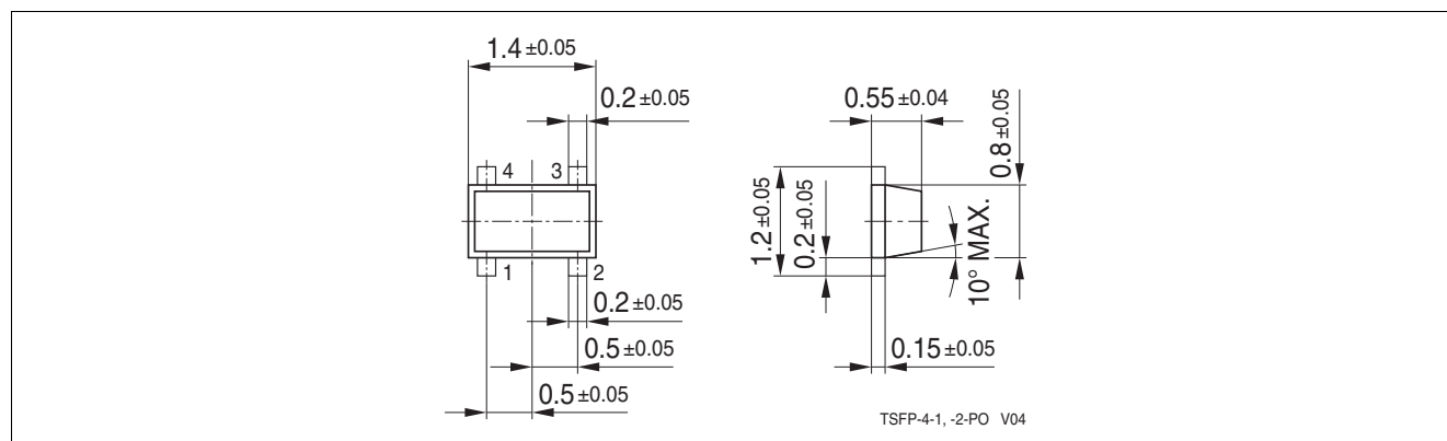
Figure 7-1 Package Outline
