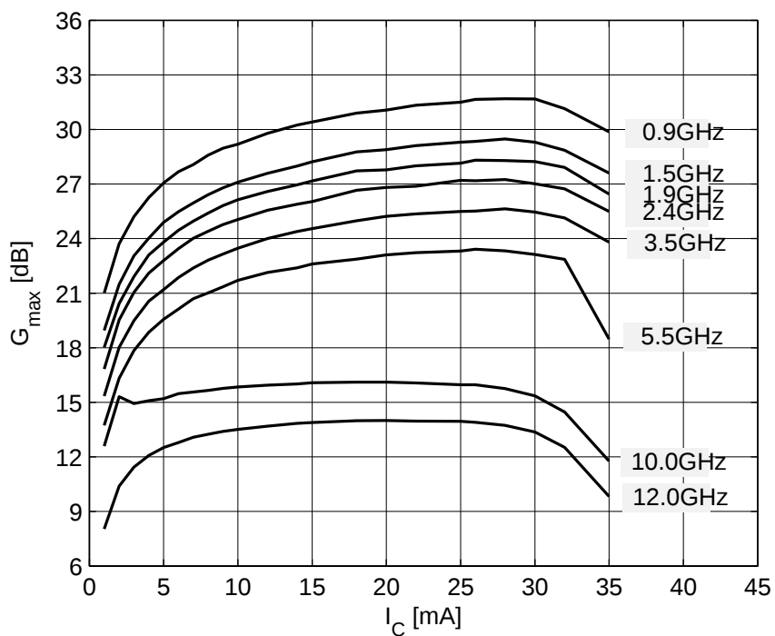
Figure 5-13 Maximum Power Gain G_{\max} = f(I_C) , V_{CE} = 1.8 \text{ V} , f = \text{Parameter in GHz}
