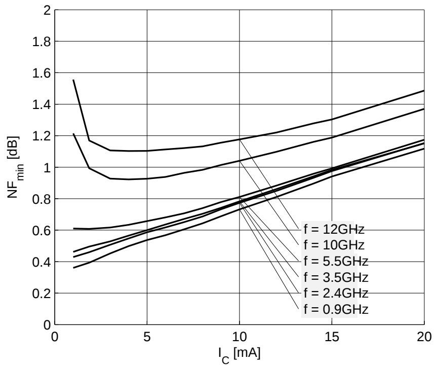
Figure 5-19 Noise Figure NF_{min} = f(I_C) , V_{CE} = 1.8 V, Z_S = Z_{opt} , f = Parameter in GHz
