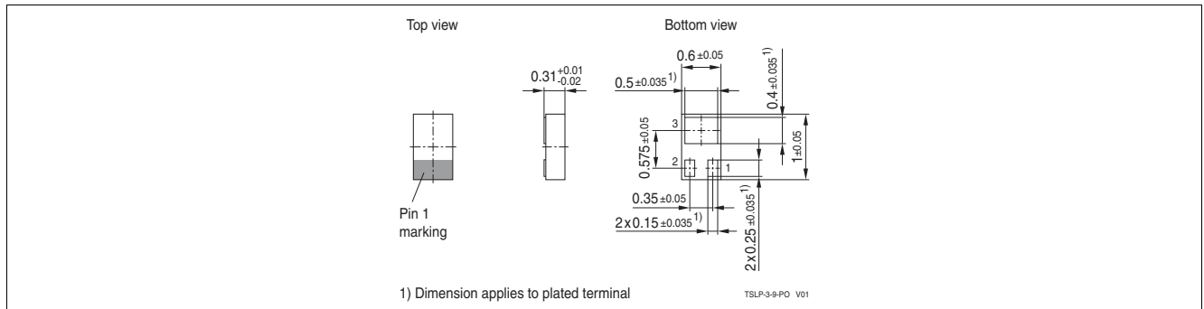
Figure 7-1 Package Outline
