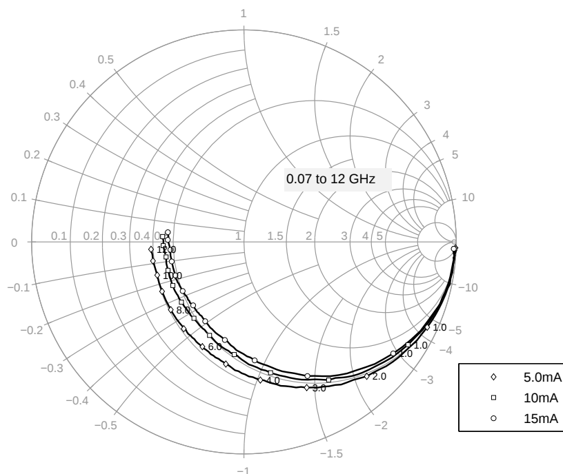
Figure 5-17 Output Reflection Coefficient S_{22} = f(f) , V_{CE} = 1.8\text{ V} , I_C = 5 / 10 / 15\text{ mA}
