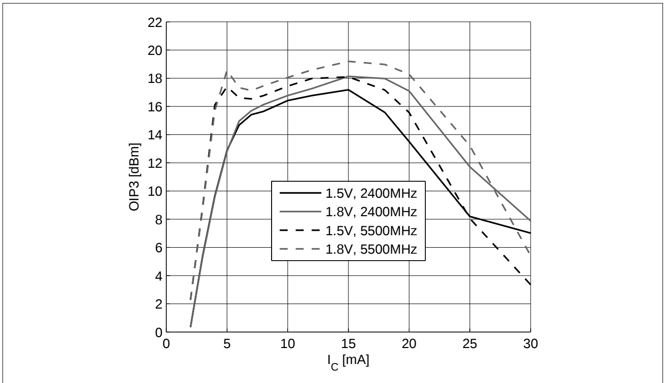
Figure 5-8 3rd Order Intercept Point at output OIP3 = f(I_C) , Z_S = Z_L = 50 \Omega , V_{CE}, f = \text{Parameter}
