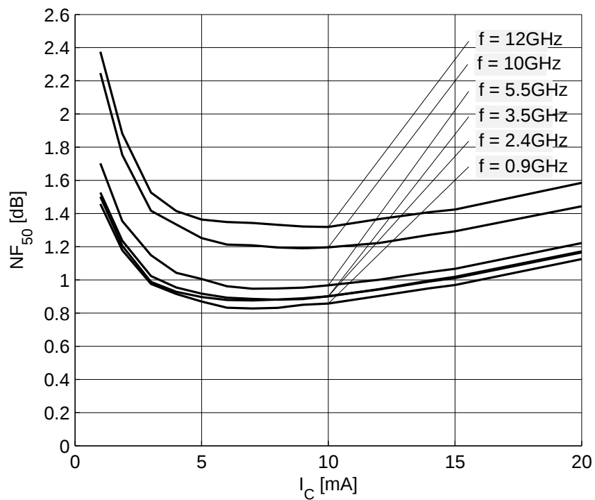
Figure 5-20 Noise Figure NF_{50} = f(I_C) , V_{CE} = 1.8 V, Z_S = 50 \Omega , f = Parameter in GHz
