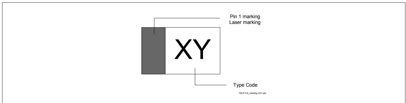
Figure 7-3 Marking Description (Marking BFR840L3RHESD: T8)
