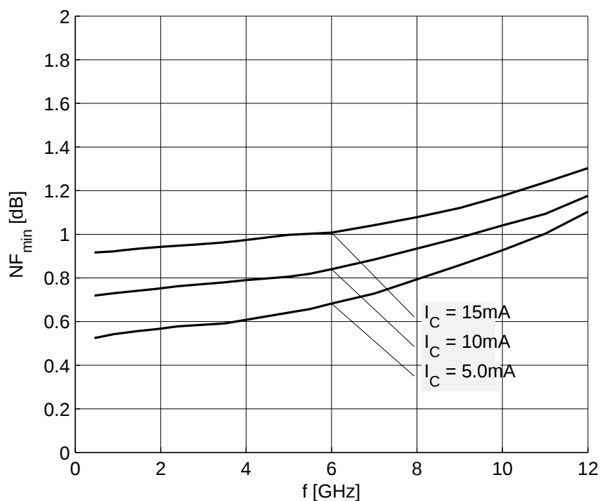
Figure 5-18 Noise Figure NF_{min} = f(f) , V_{CE} = 1.8\text{ V} , I_C = 5 / 10 / 15\text{ mA} , Z_S = Z_{opt}
