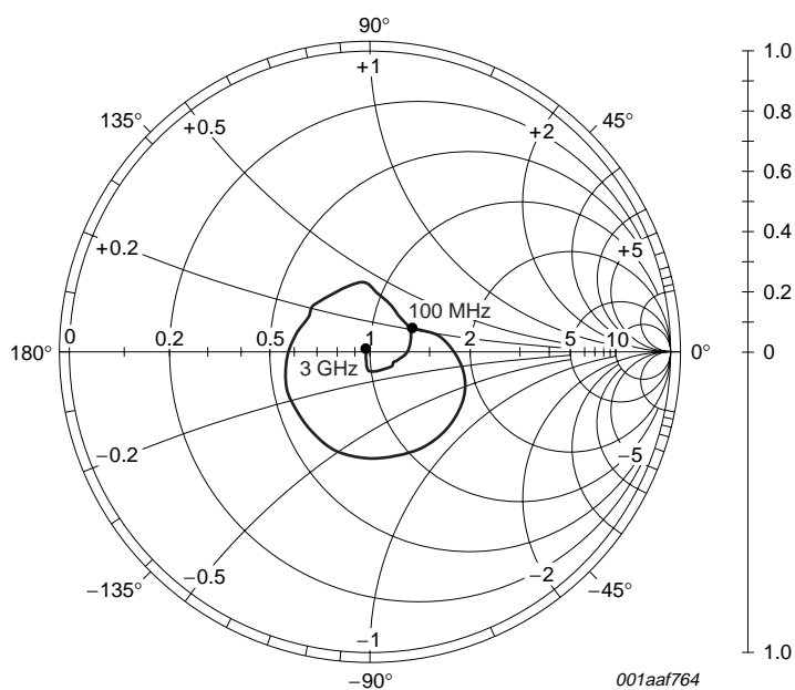
Fig 4. Input reflection coefficient ( S_{11} ); typical values
