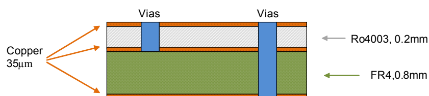
BGA825L6S_application_board_sideview.vsd
