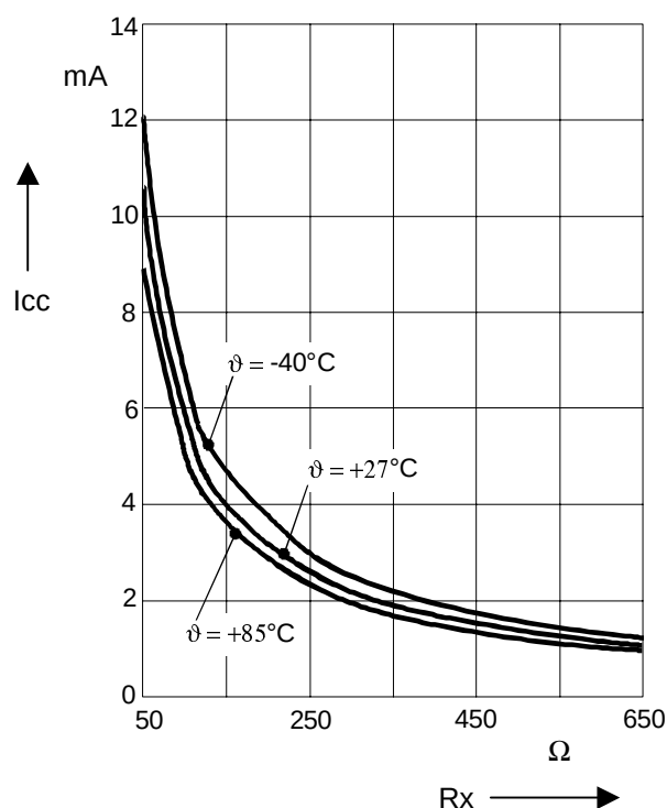
Device Current versus Rx and Temperature V cc =3V
