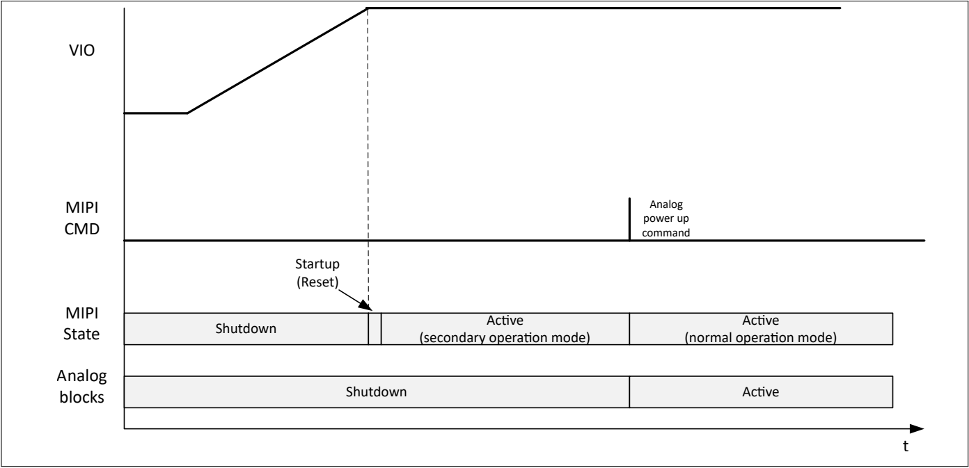
Figure 1: Startup Timing Diagram
