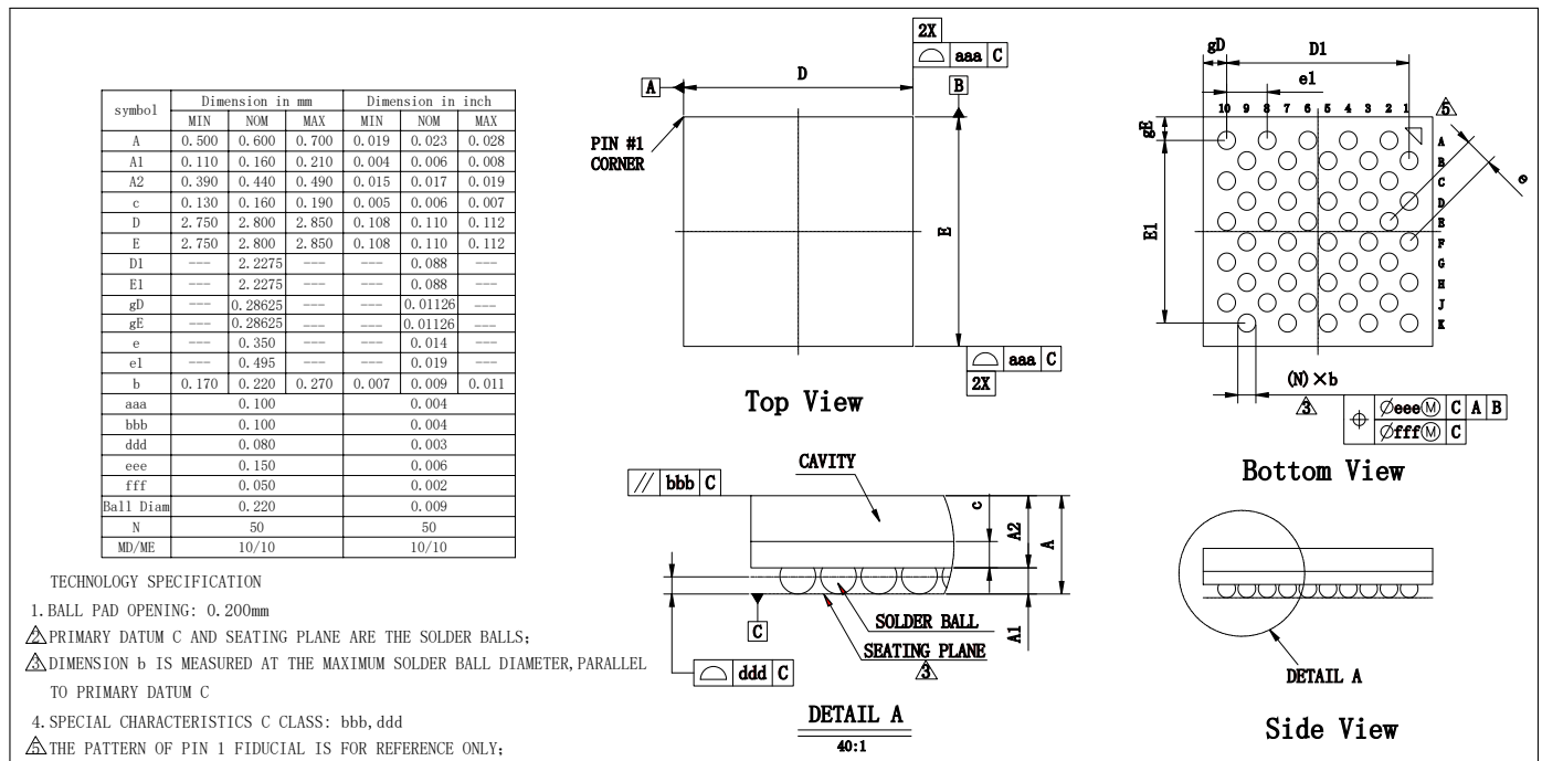
Figure 5: PG-WF2BGA-50-1 Package Outline (top and side views)
