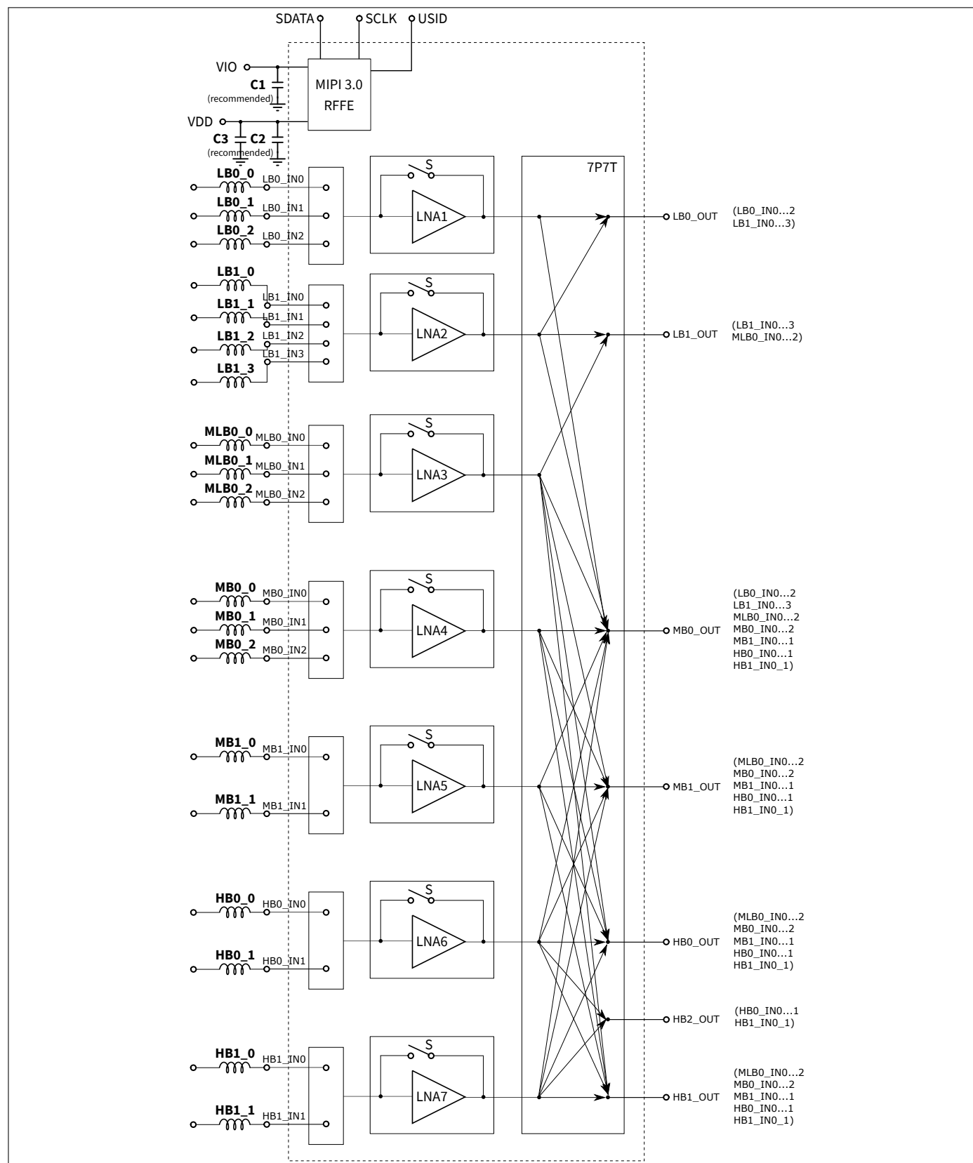
Figure 4: BGM687U50 Application Schematic
