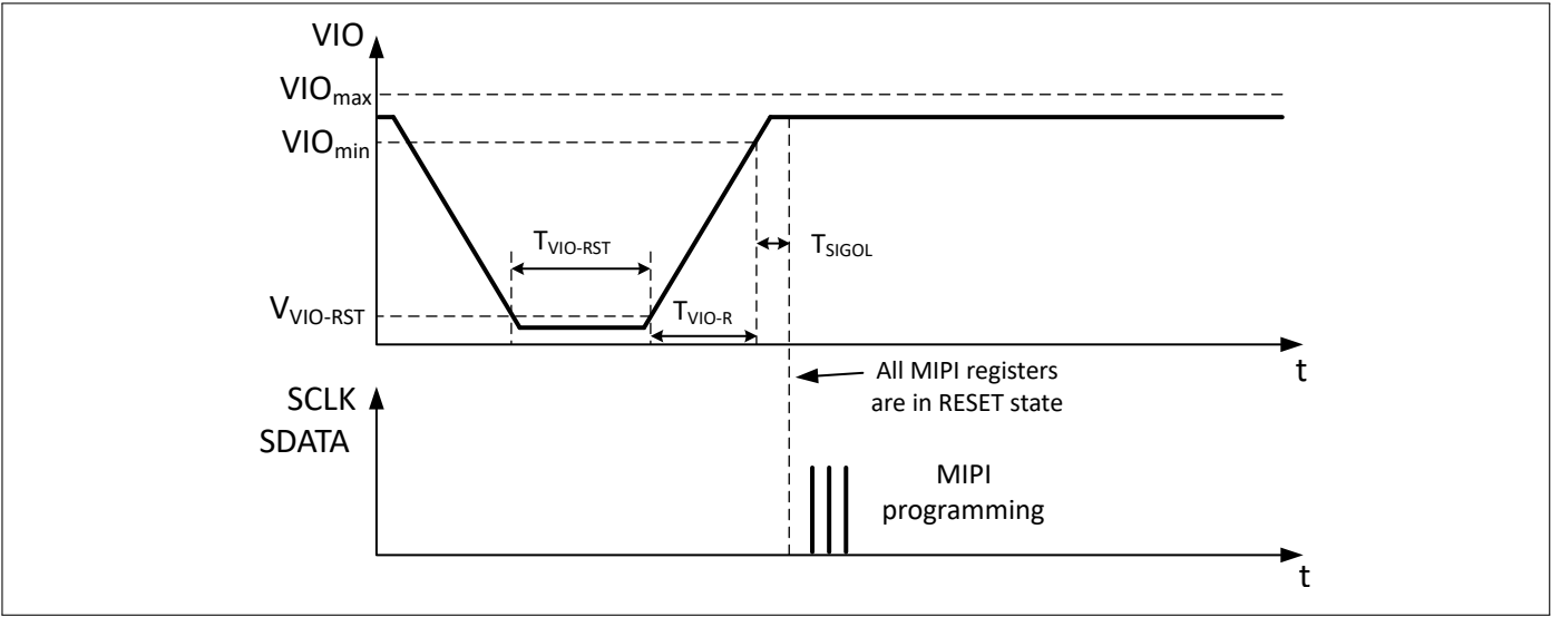
Figure 2: V_{IO} Reset Timing Diagram
