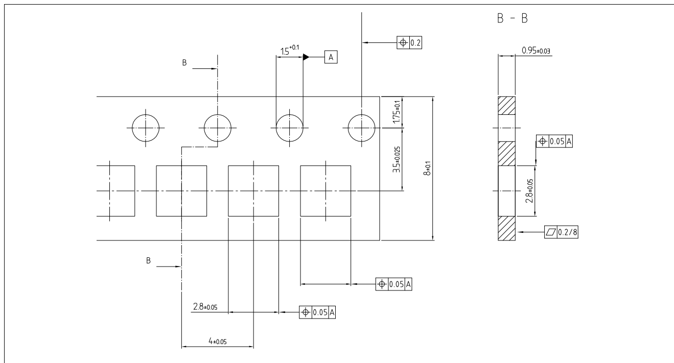
Figure 9 TSNP-11-2 carrier tape
