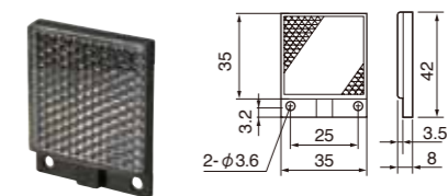
Small reflector V-42
