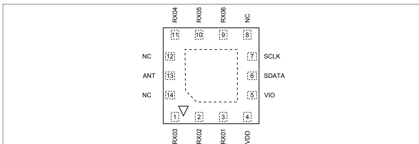
Figure 9: Pin configuration (top view)
