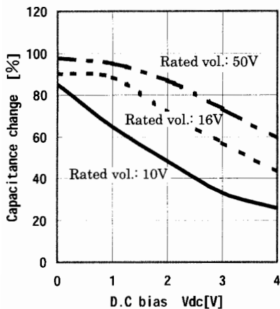
Fig.25 Capacitance change-Bias characteristic (F type) (Reference)
