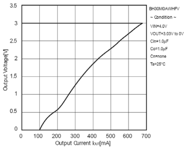
Figure 5. Output Voltage vs. Output Current (OCP Threshold)
