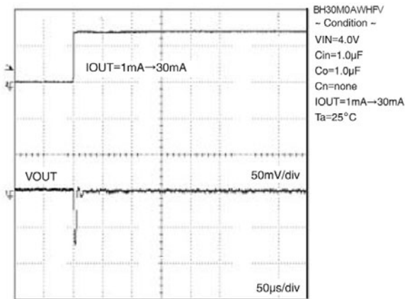
Figure 9. Load response
