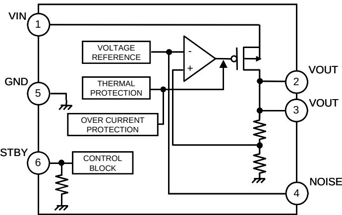
Figure 2. Block diagram
