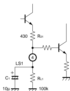
Fig.8 Suppressing phase detecting circuit
