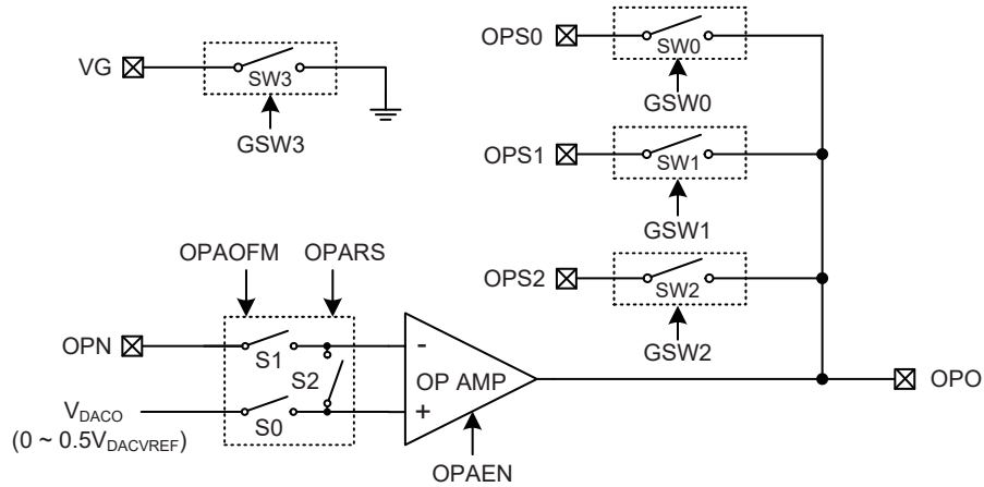
Operational Amplifier Structure
