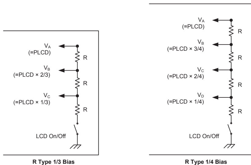
R Type Bias Voltage Generation
