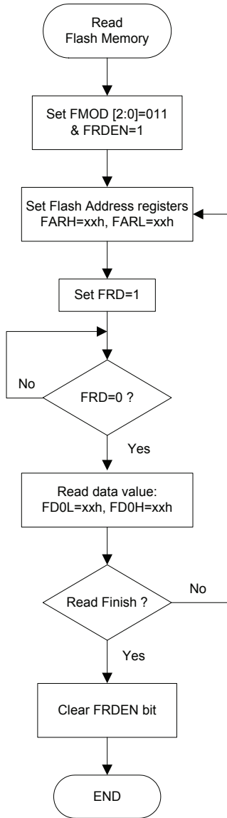
Read Flash ROM Procedure
