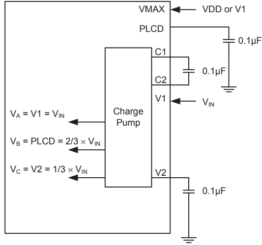
Power Supply from pin V1
