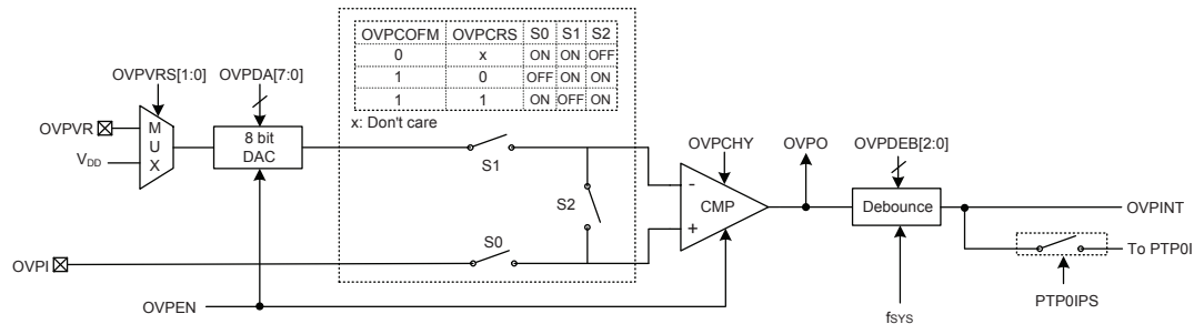
Over Voltage Protection Circuit
