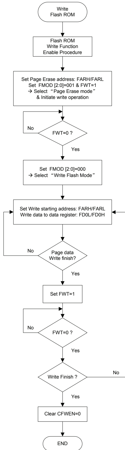
Write Flash ROM Procedure
