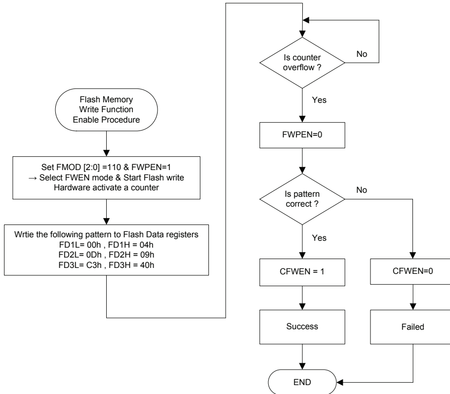
Flash ROM Write Function Enable Procedure
