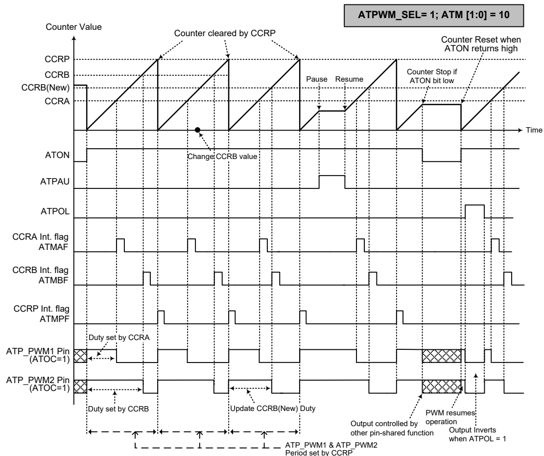
ATM Audio PWM Output Mode – Change CCRB Value
