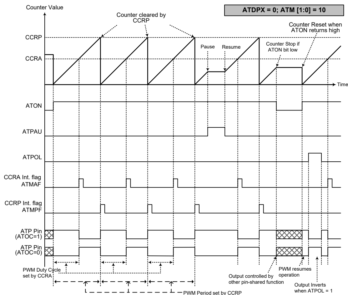
ATM Normal PWM Output Mode – ATDPX=0
