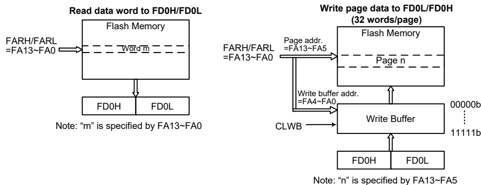
Flash Memory IAP Read/Write Structure – BH67F5265
