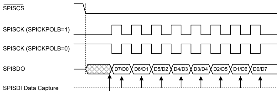
SPI Master Mode Timing
