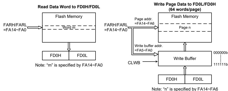
Flash Memory IAP Read/Write Structure – BH67F5275
