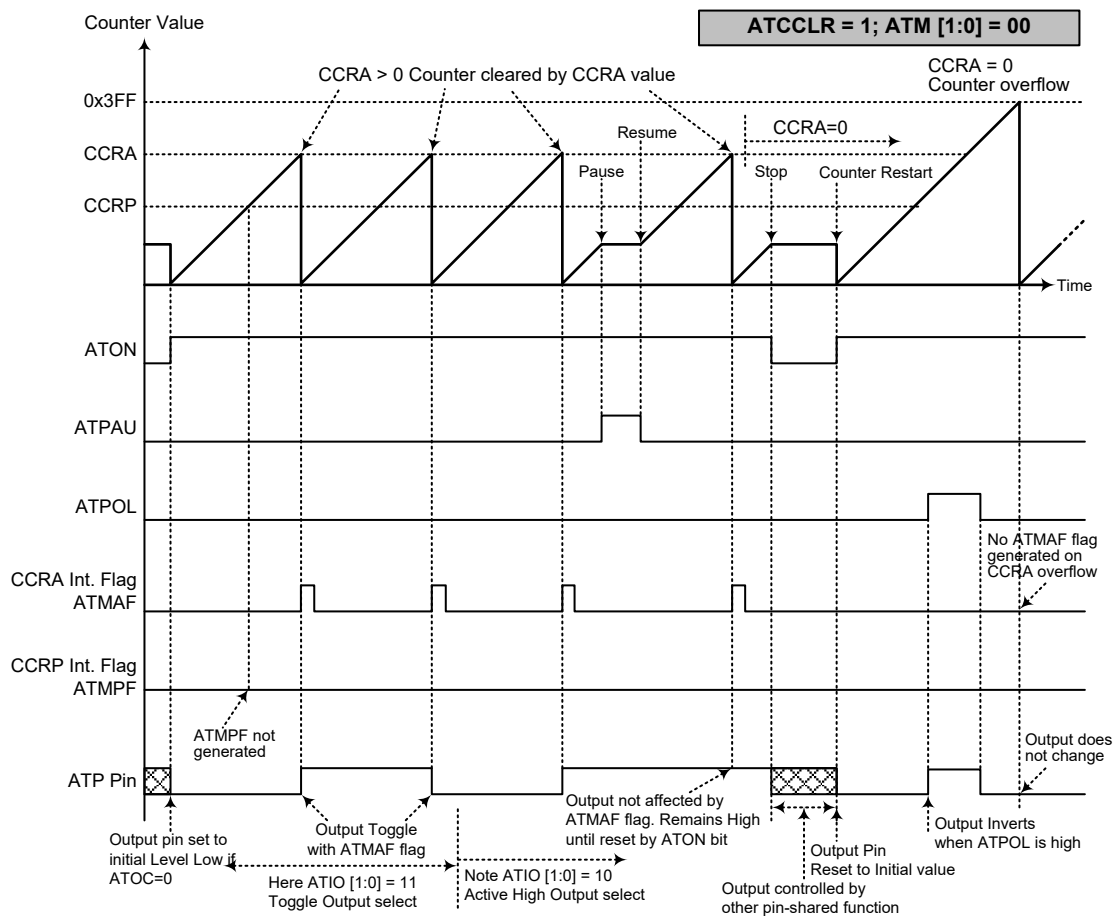
Compare Match Output Mode – ATCCLR=1
