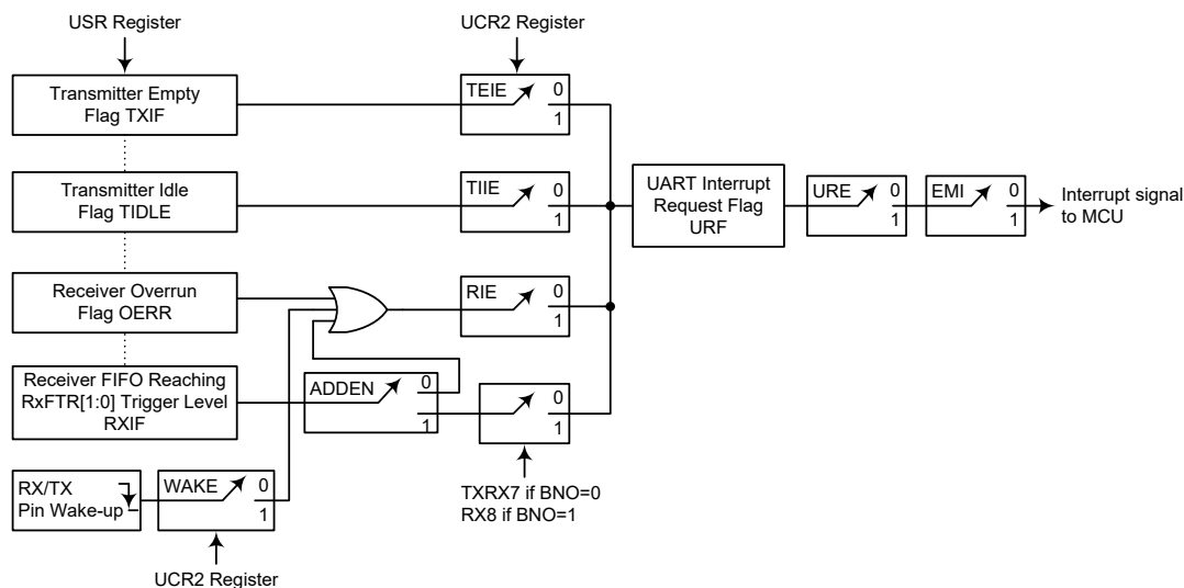
UART Interrupt Structure
