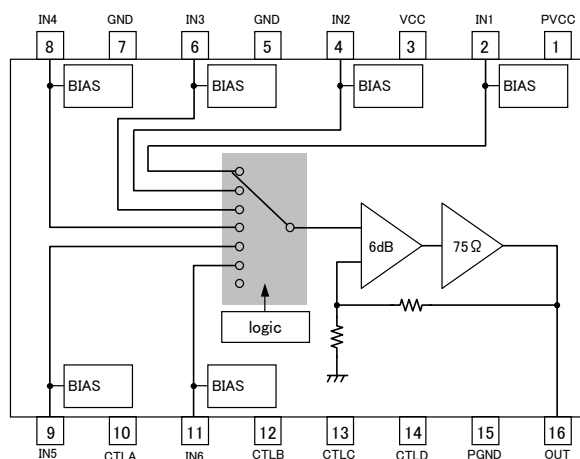
Fig.2 BH76361FV
