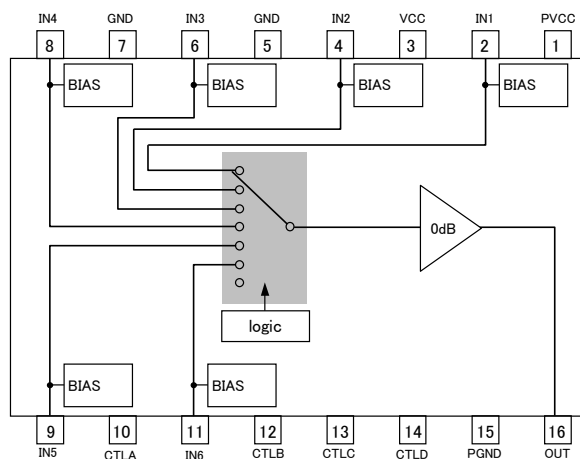
Fig.4 BH76363FV
