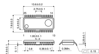
HSOP25
