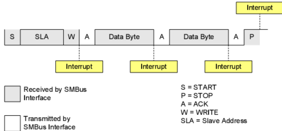
Figure 32 SMBUS Slave Receiver Sequence
