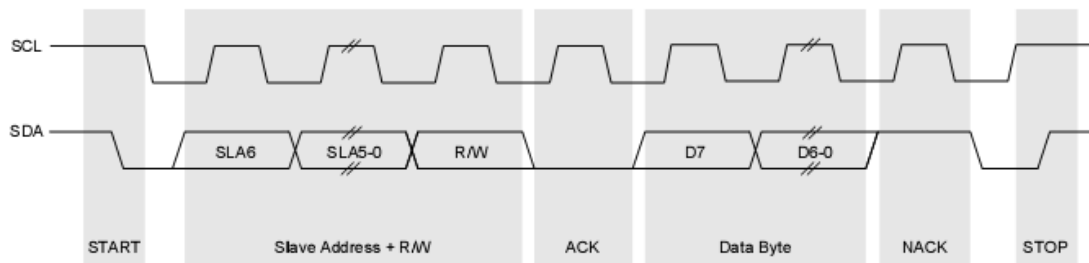
Figure 28 SMBUS Transaction
