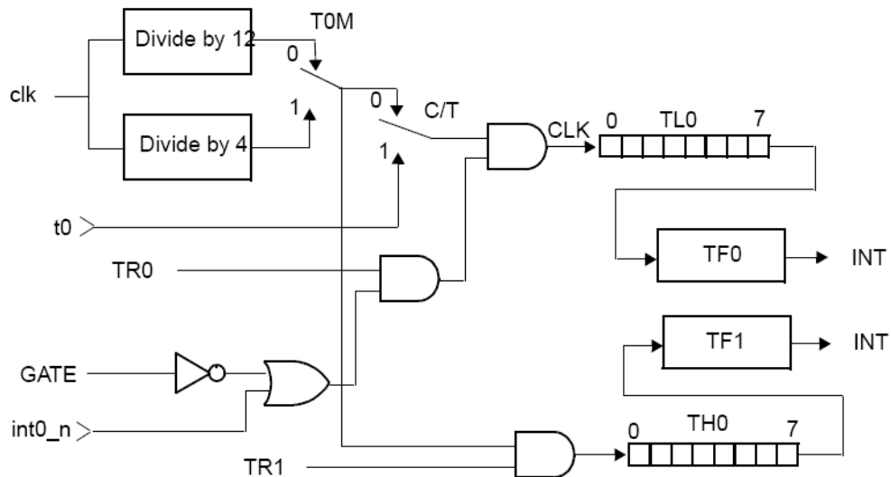
Figure 12 Timer 0 – Mode 3
