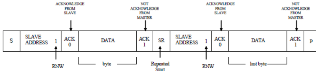
Figure 25 Repeated Start or Stop condition after last byte
