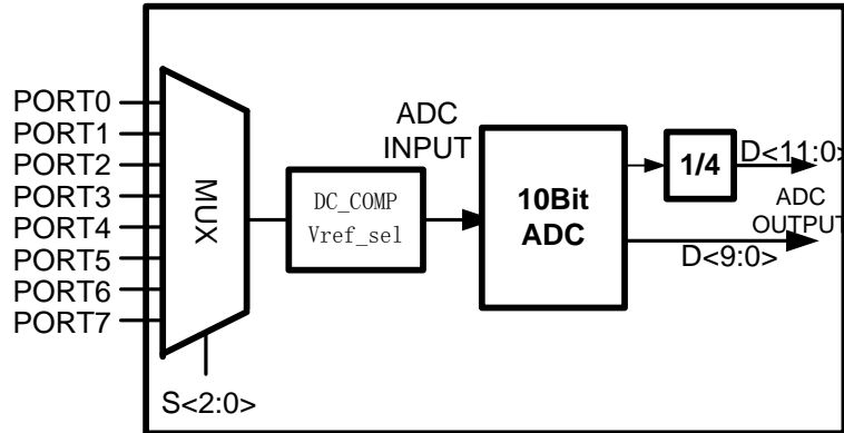
Figure 14 ADC
