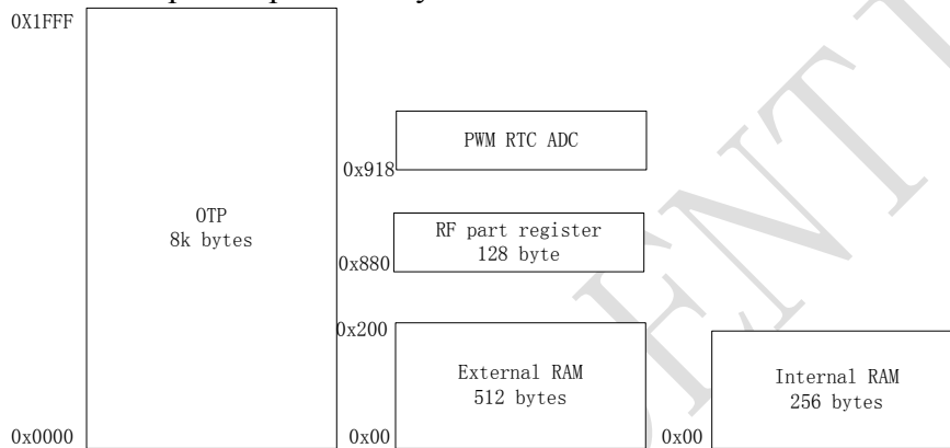
Figure 5 FLIP51 SPACE
