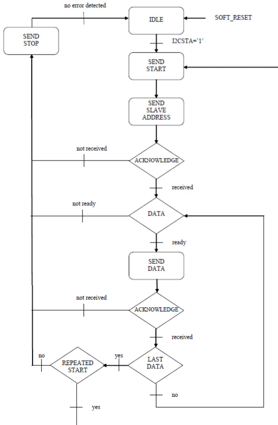
Figure 23 Transmission FSM
