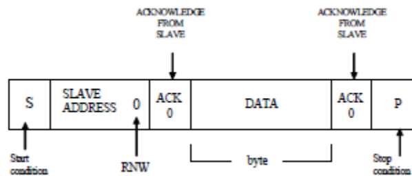
Figure 21 Typical transmission
