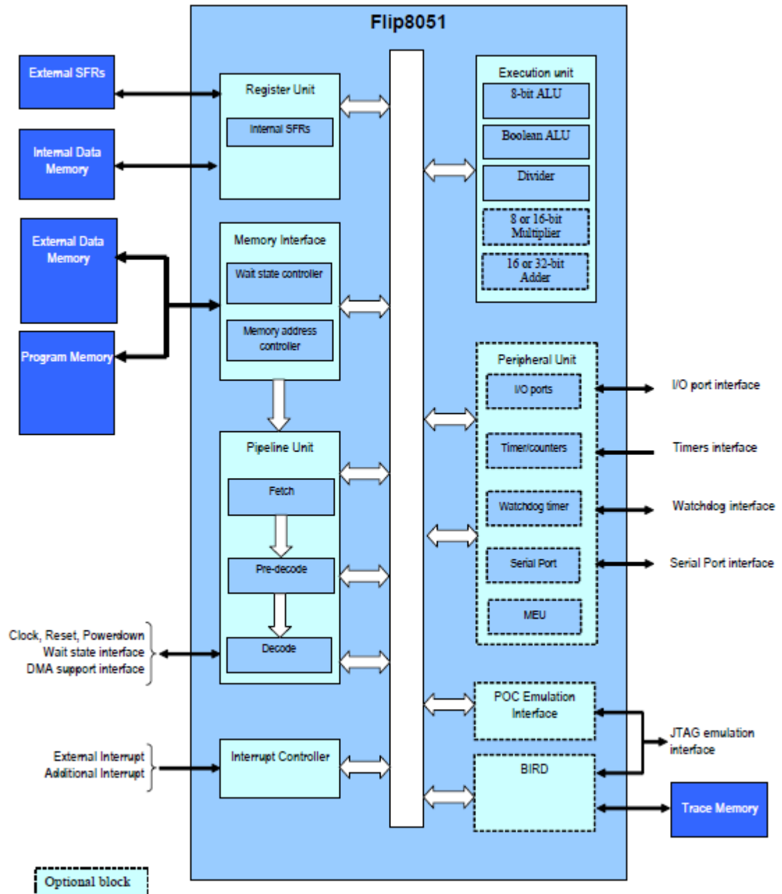
Figure 4 FIIP51 architecture
