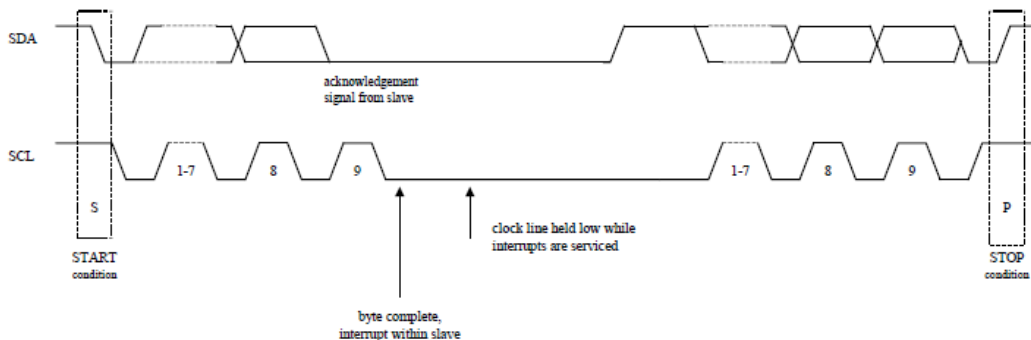
Figure 30 Clock synchronization
