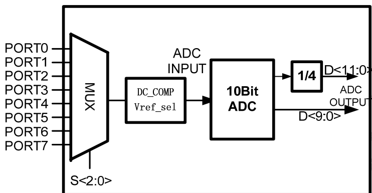
Figure 14 ADC block
