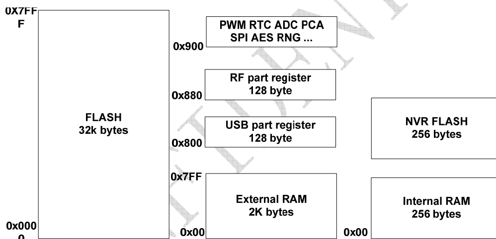
Figure 5 FLIP51 Space
