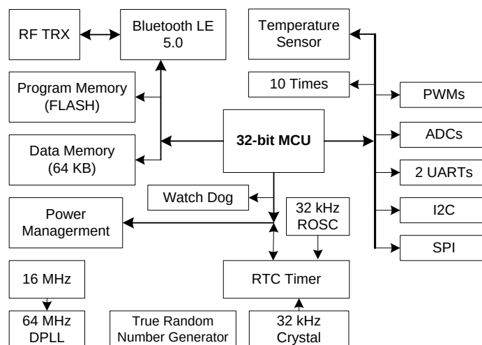
Figure 1 BK3431Q Block Diagram
