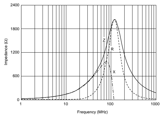
BLM18BD182SN1
