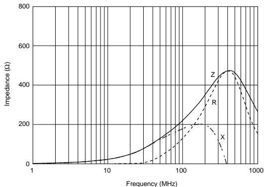
BLM18BD221SN1
