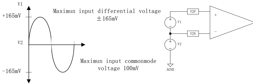
Figure 4. Voltage Channels
