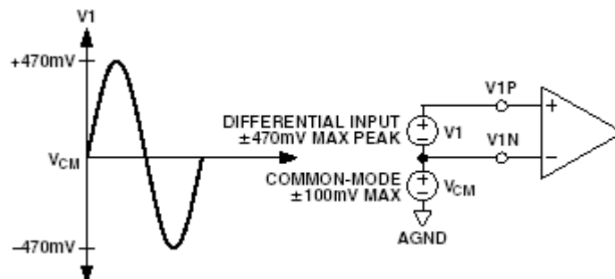
Figure 22. Maximum Signal Levels, Channel 1, Gain=1
