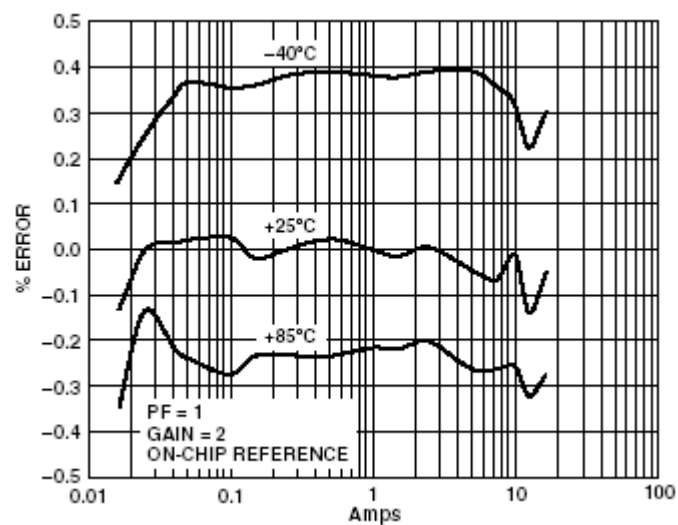
Figure 2. Error as a% of Reading (Gain=1)
