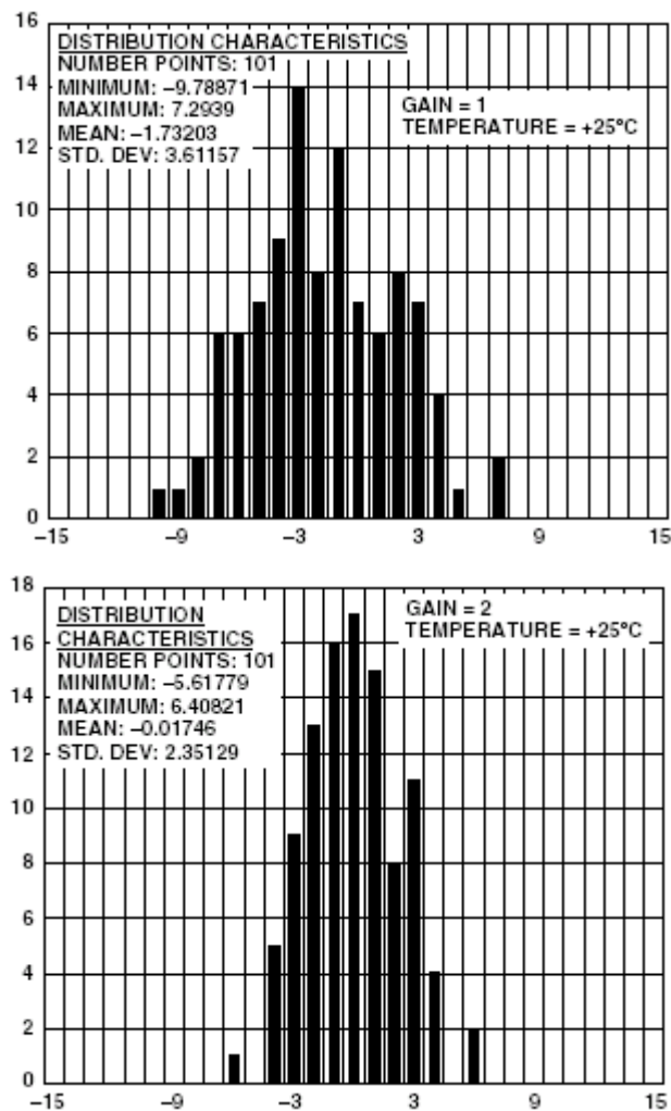
Figure 14. Channel 1 Offset Distribution (Gain=1)
