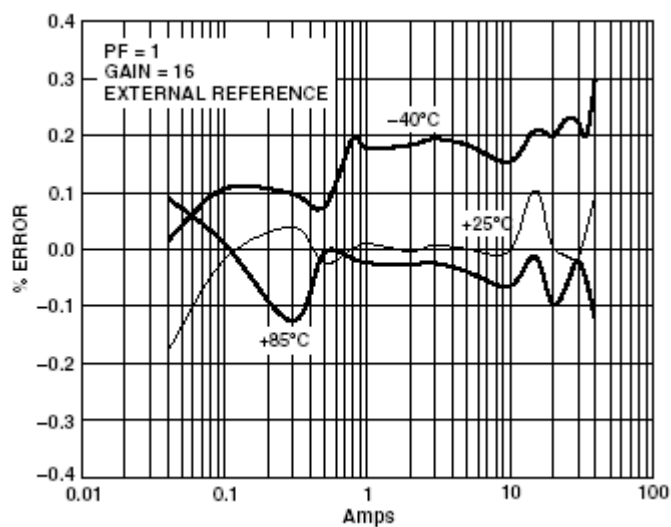
Figure 10. Error as a% of Reading over Temperature Figure 11. Error as a% of Reading over Temperature
