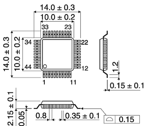
44-Lead Plastic Quad Flatpack Package [QFP]
