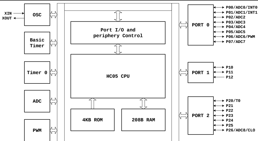
Block Diagram
