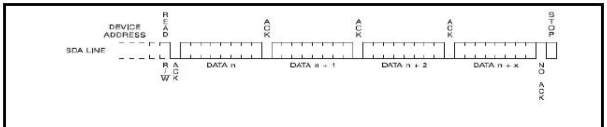
Figure 9. Sequential Read
