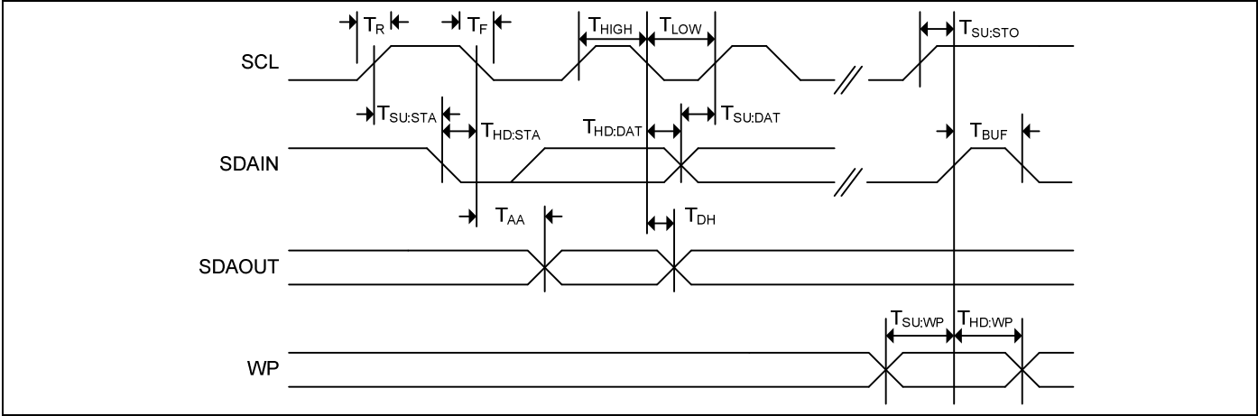
Figure 1-11. Bus Timing
