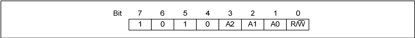
Figure 1-5. Slave Address
