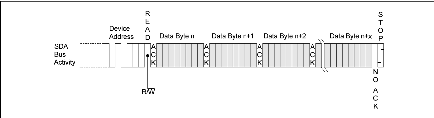
Figure 1-10. Sequential Read
