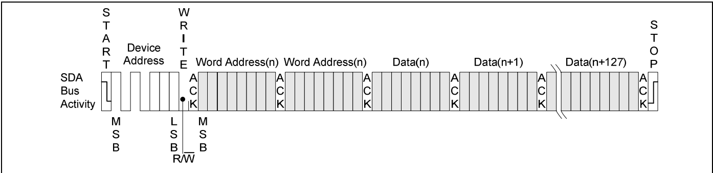
Figure 1-7. Page Write
