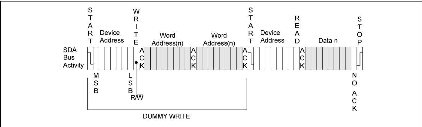
Figure 1-9. Random Address Read
