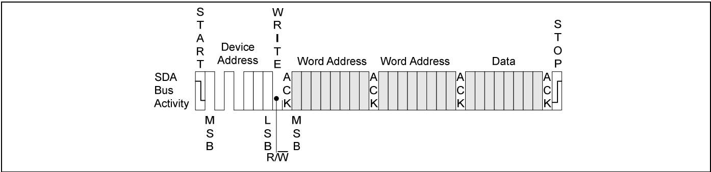
Figure 1-6. Byte Write
