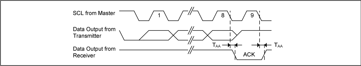
Figure 1-2. output Acknowledge
