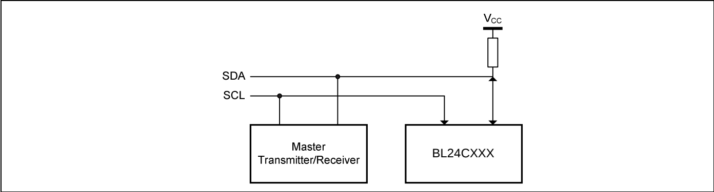
Figure 1-1. Typical System Bus Configuration
