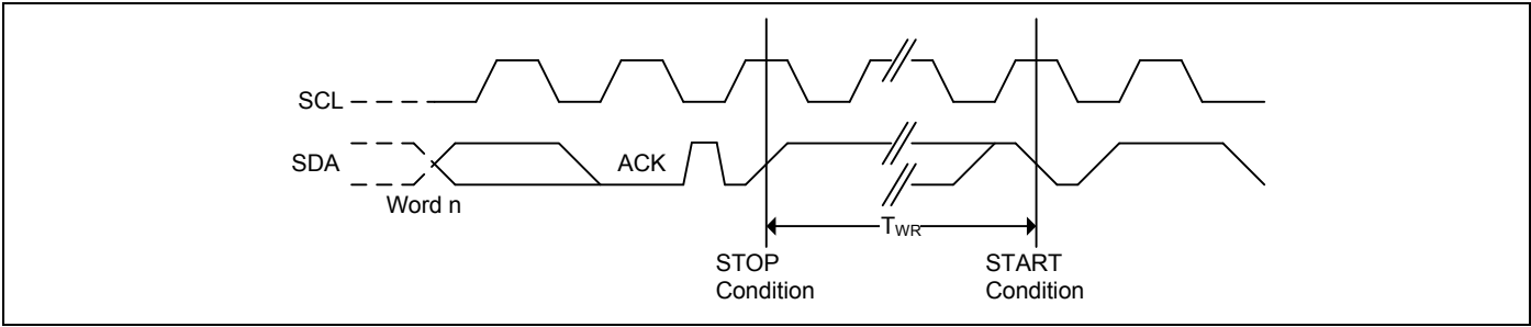
Figure 1-12. Write Cycle Timing
