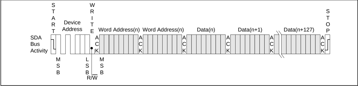
Figure 1-7. Page Write
