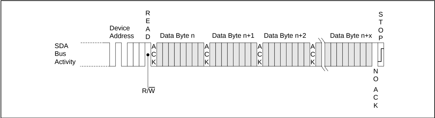
Figure 1-10. Sequential Read
