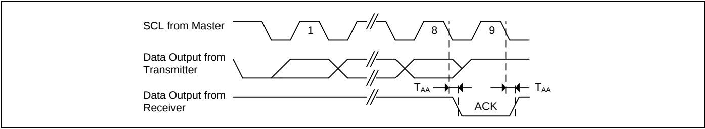
Figure 1-2. output Acknowledge
