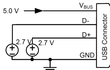
Fig 2. Divider 3 DCP
