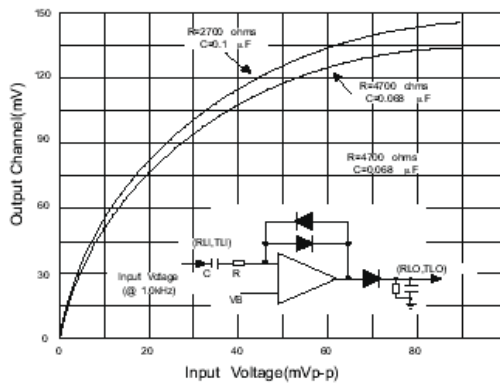
Fig 8 Log Amp Transfer Characteristics
