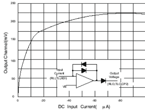
Fig 7 Log Amp Transfer Characteristics
