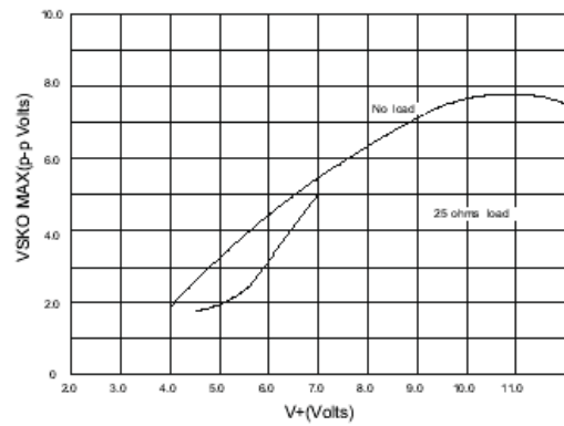
Fig 9 Speaker Amp Output vs Supply Voltage
