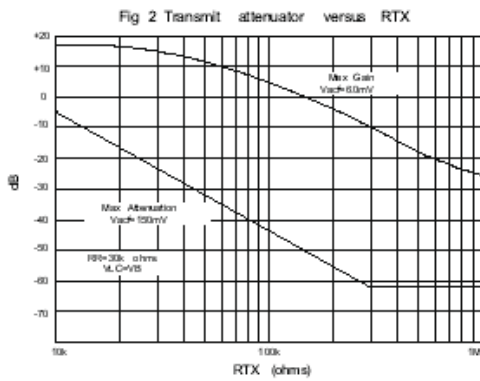
Fig 2 Transmit attenuator versus RTX
