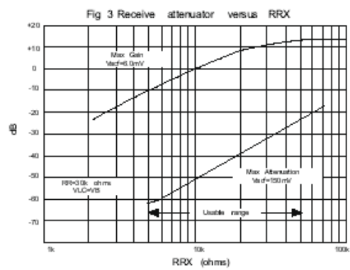
Fig 3 Receive attenuator versus RRX
