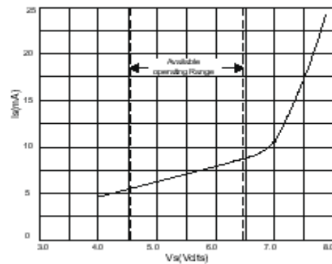
Fig 15 Supply Current vs Supply Voltage
