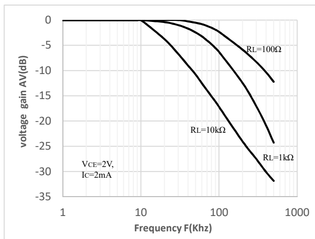
Fig.10 Frequency Response
