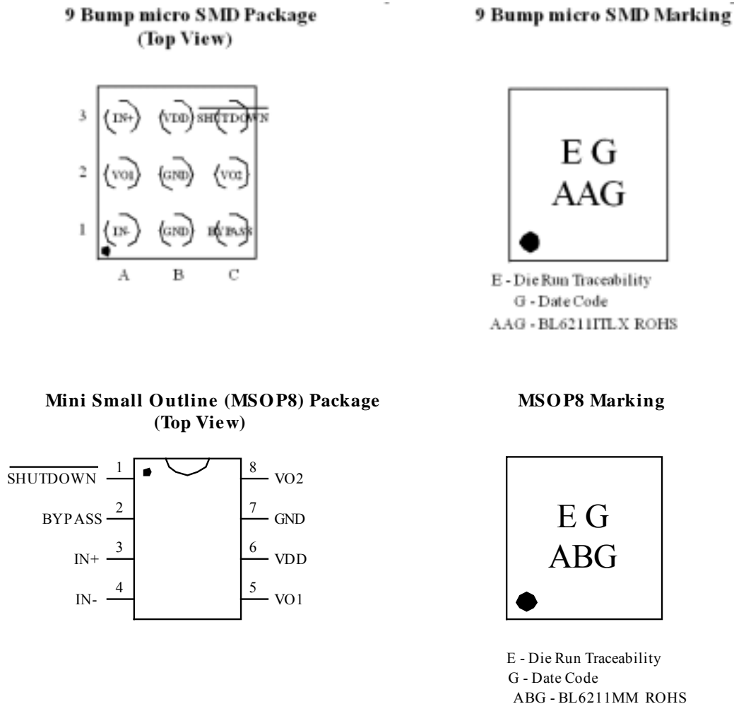
Figure 2 Pin Diagram of BL6211
