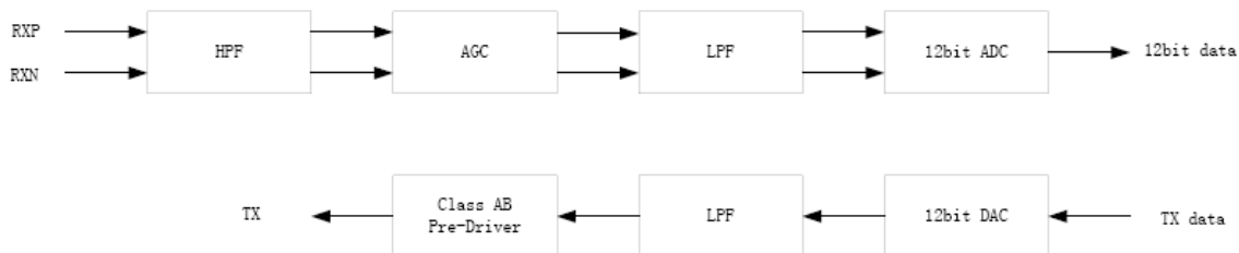
BL6810 Analog Front End
