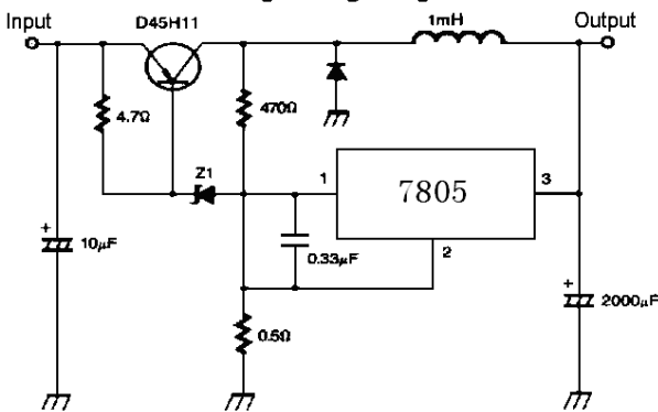
Switching Regulator
