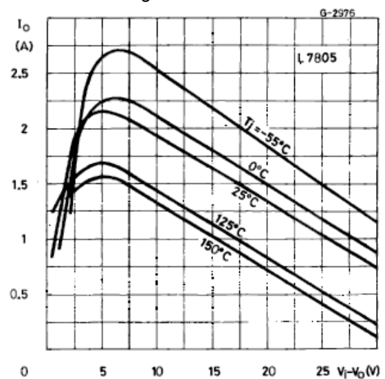
Figure 2: Peak Output Current vs Input/output Differential Voltage
