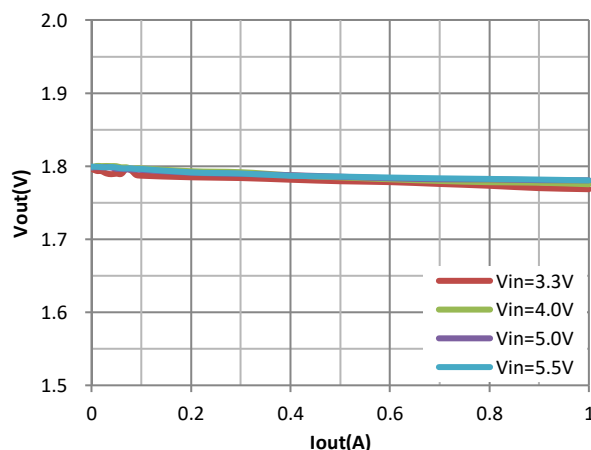
Load Regulation ( V_{out}=1.8\text{V} )
