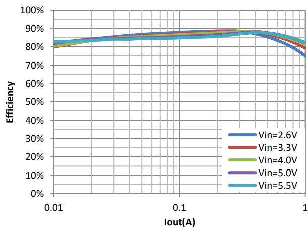
Efficiency ( V_{out}=2.5\text{V} )
