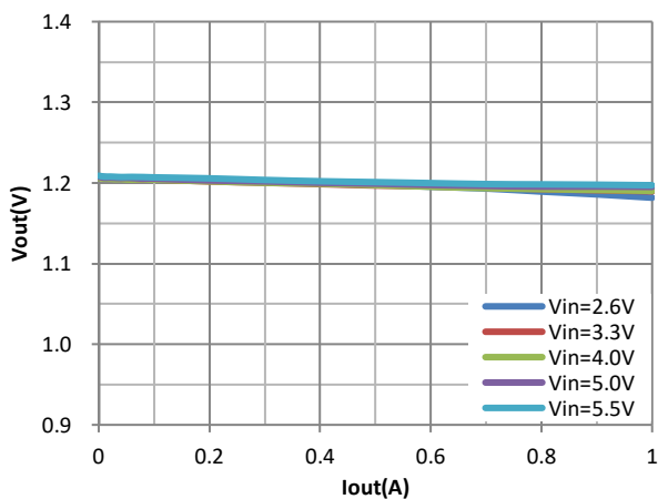
Load Regulation ( V_{out}=1.2\text{V} )
