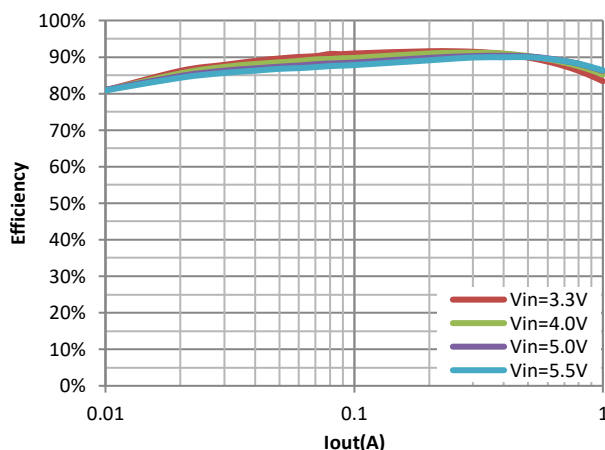
Efficiency ( V_{out}=3.3\text{V} )
