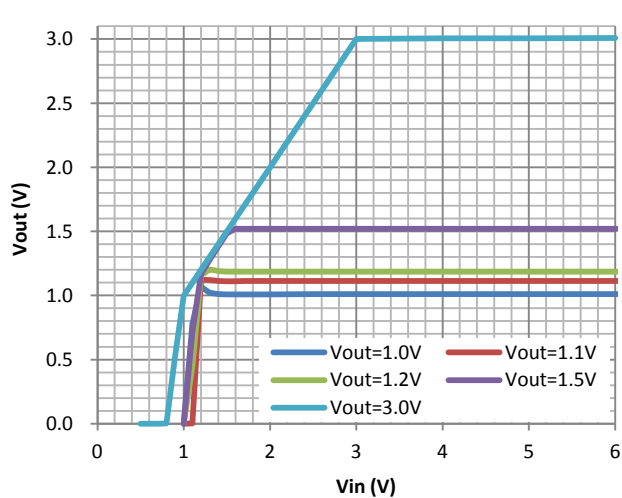
Line Regulation
