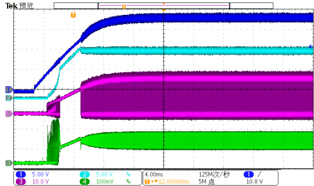
Start-up Waveform with EN=VIN VIN=18V, VOUT=12V, IOUT=125mA, L=47uH CH1 (VIN), CH2 (VOUT), CH3 (LX), CH4 (IL)
