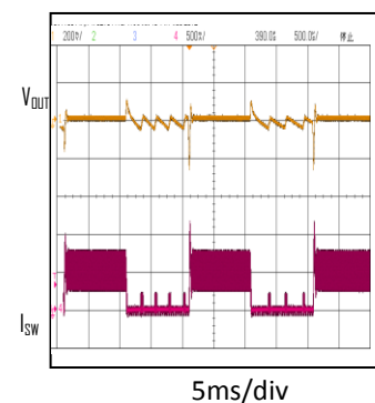
Load Transient Response VIN=12V,VOUT=3.3V,IOUT=0 to 0.5A
