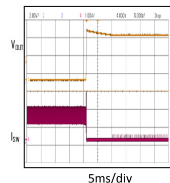
Short-Circuit Recovery VIN=24V,VOUT=5V,IOUT= Short to 0A
