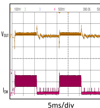
Load Transient Response VIN=12V,VOUT=5V,IOUT=0 to 0.5A
