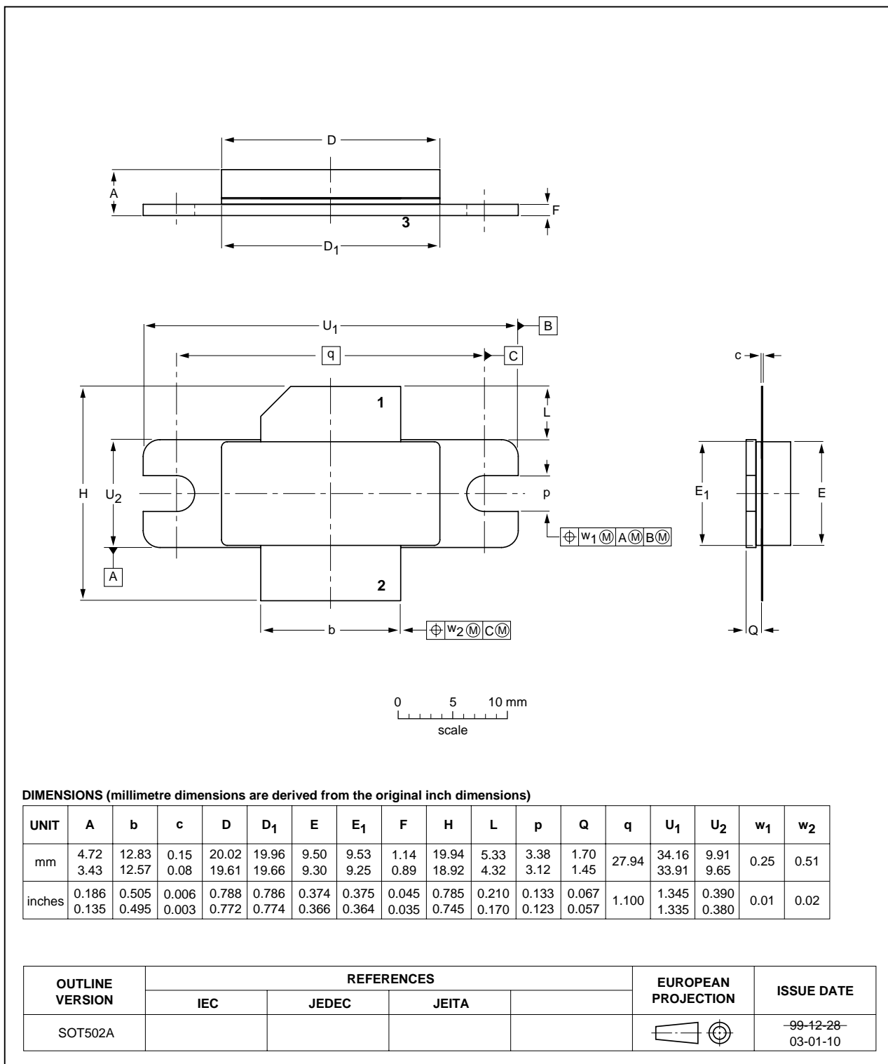
Fig 9. Package outline SOT502A
