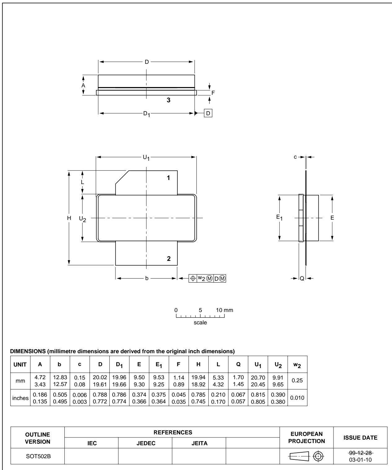
Fig 10. Package outline SOT502B
