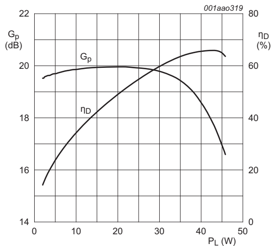
Fig 5. Power gain and drain efficiency as a function of average power; typical values
