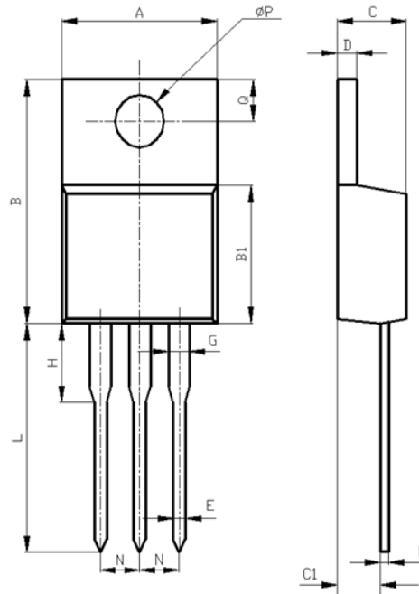
TO-220 Package
