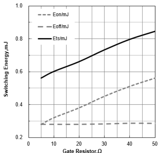
Figure 16. Typical Switching Energy vs Gate Resistor (T J =25°C, V CE =400V, V GE =15/0V, I C =20A)
