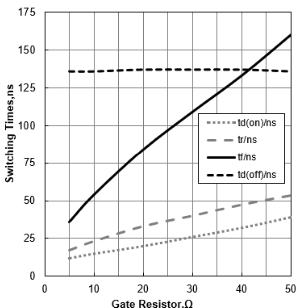
Figure 15. Typical Switching Times vs Gate Resistor (T J =25°C, V CE =400V, V GE =15/0V, I C =20A)
