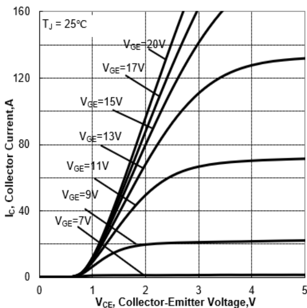
Figure 7. Typical Output Characteristics ( T_J=25^{\circ}C )
