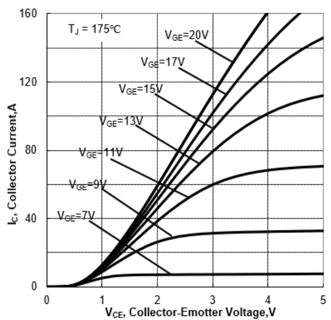
Figure 8. Typical Output Characteristics ( T_J=175^{\circ}C )
