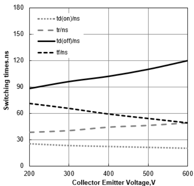
Figure 19. Typical Switching Times vs V_{CE} ( T_J=25^\circ\text{C} , V_{GE}=15/0\text{V} , I_C=50\text{A} )
