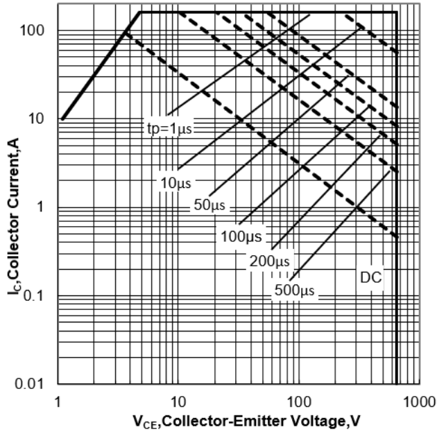
Figure 1. Forward Bias Safe Operating Area for TO247/TO3PN
